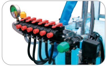
Pressure regulator valve at 6 ways, with electric general ON/OFF valve and switch box
